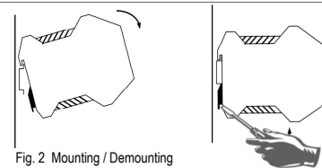
Fig. 2 Mounting / Demounting
