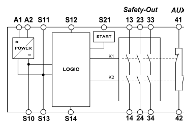
Fig. 1 Block diagram SR3A
