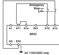
Fig. 4: Two-channel emergency stop circuit with short circuit and earth fault monitoring. (category 4, up to PL e)
