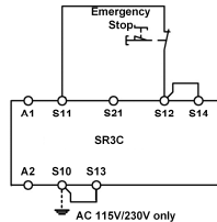
Fig. 6: Single-channel emergency stop circuit with earth fault monitoring. (category 1, up to PL c)
