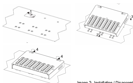
Image 2: Installation / Disassembly
