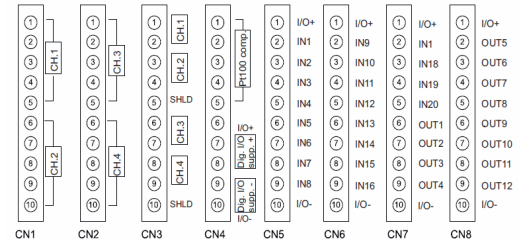
Image 4: Pin assignment
