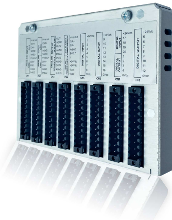
Image 1: Plug-In I/O-Module
